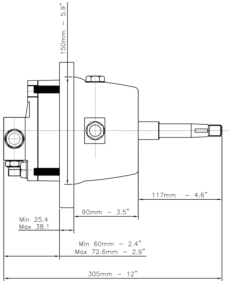
UP56, UP68 REAR MOUNT
