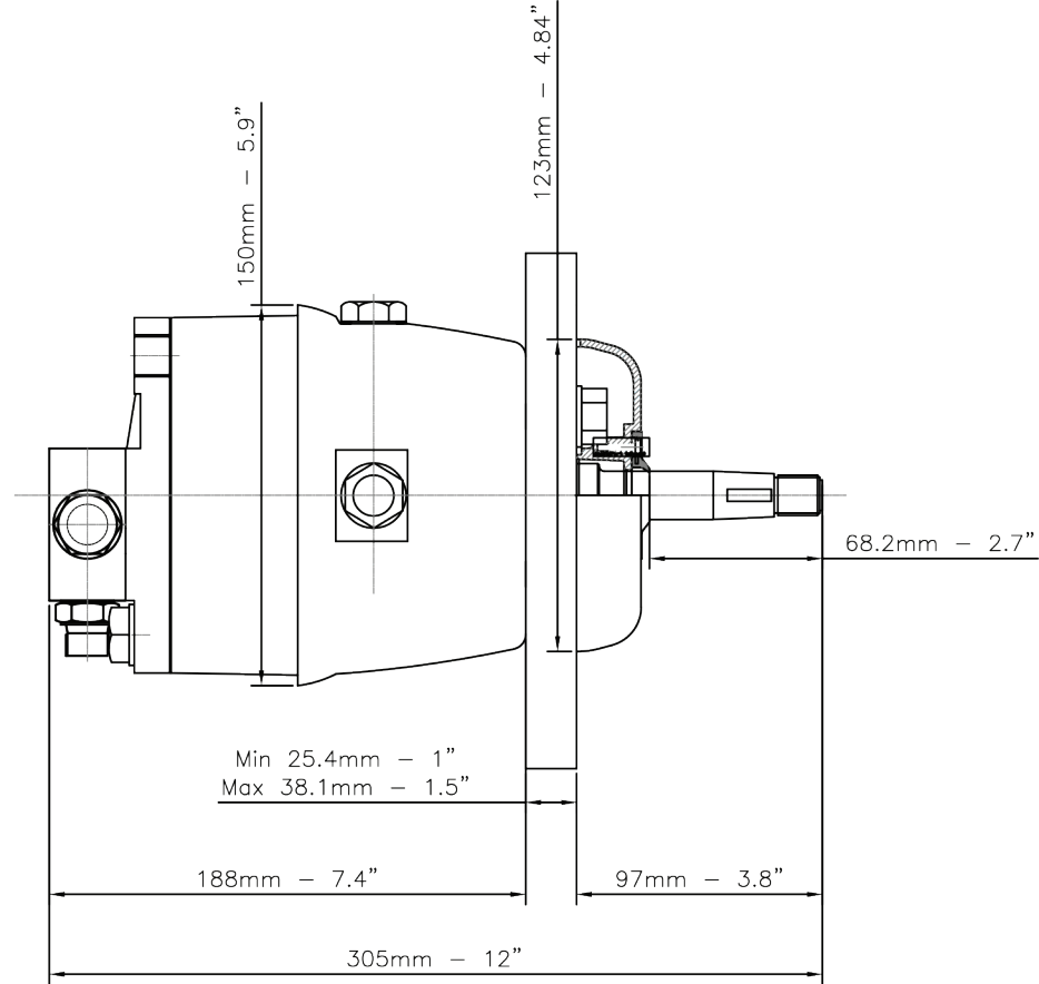
UP56, UP68 INTERMEDIATE MOUNT
